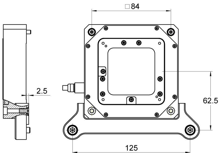
P-733.AP1, dimensions in mm
